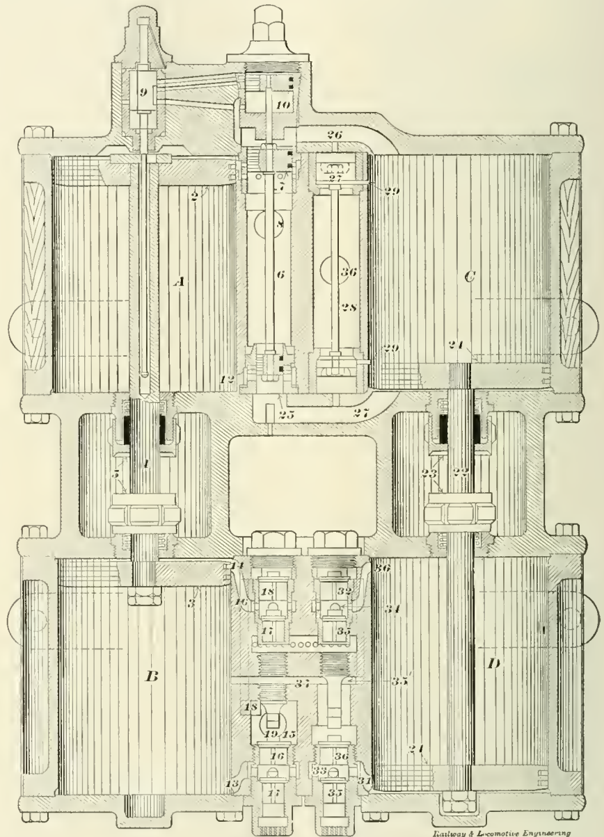
MARSH'S COMPOUND AIR PUMP.
